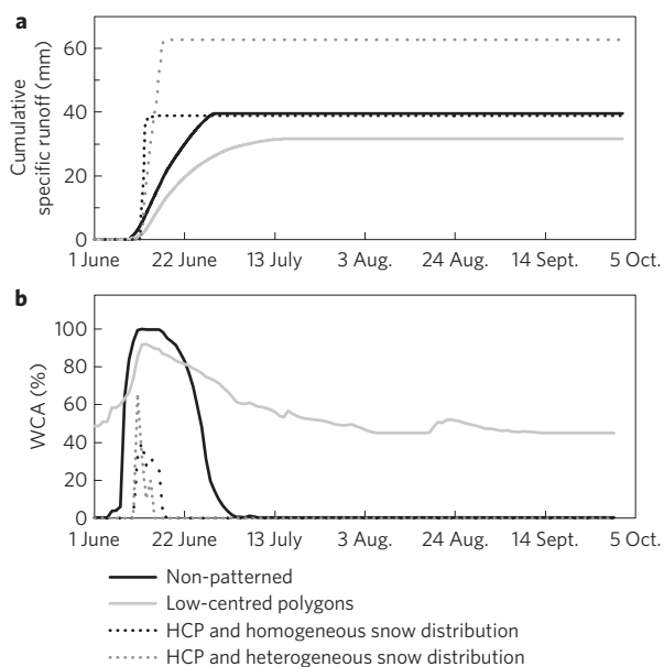
Figure 6 | Model experiments of runoff and inundation using differing polygon types and snow distribution. a,b , Simulated runoff (a) and water covered area (WCA, b) from the four scenarios; a non-patterned ground basin (solid black line), a watershed dominated by LCPs (solid grey line), and HCPs with connected troughs, with deeper snow accumulation in troughs versus mounds (grey dotted line) and a spatially homogeneous end-of-winter snow distribution (black dotted line). End-of-winter snow water equivalent is identical (119 mm) among the four scenarios. LCPs promote lower runoff and extensive inundation, whereas the development of troughs and the subsequent increased spatial variability in snowcover increases runoff and decreases WCA. Note the lack of increased runoff when snow is homogeneously distributed over the HCPs.
