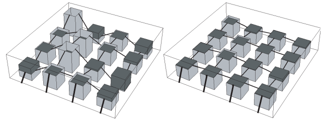
Fig. 4. Model principles to describe hillslope outflow. Each site has a storage capacity to retain water. In the left figure, the capacity values c of the sites are random numbers between 0.0 and 1.0 and are shown in light gray. All sites received the same amount of water r during the storm (dark gray boxes). In this example, r equals 0.5. The volume of the water above the capacity value corresponds to the water that can drain out if it is connected to the boundary at the bottom. In this example, six sites have free water that is hydraulically connected to the lower boundary of the system. In one case (top row), a site with free water is enclosed by unsaturated sites. Right: In this model, the capacity values are distributed according to a normal distribution with mean 0.5 and a standard deviation of 0.05.
