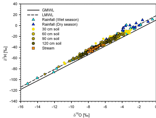
Figure 6. Isotope ( \delta^2\text{H} and \delta^{18}\text{O} ) signatures of rainfall, soil water (30, 60, 90, and 120 cm depth) and stream water. The local meteoric water line (LMWL; dashed line) is based on the 2008–2010 precipitation data and reads \delta^2\text{H} = 8.25 \cdot \delta^{18}\text{O} + 18.20 ; the solid line represents the global meteoric water line (GMWL): \delta^2\text{H} = 8 \cdot \delta^{18}\text{O} + 10 .
