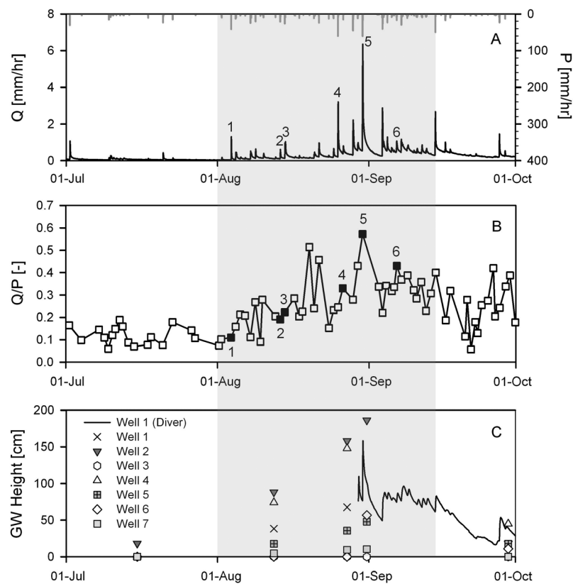
Figure 3. (a) Hourly values of rainfall (P) and streamflow (Q) as measured at the TMCF catchment from July to October 2009 and (b) the corresponding storm runoff ratios (Q/P). The numbers in Figures 3a and 3b denote the six rain storms analyzed using the various hydrograph separation techniques (see text). (c) Readings of groundwater levels for the seven wells installed in the investigated hillslope (symbols). The line shows hourly values of groundwater height for Well 1 as measured from 31 August to 1 October 2009. The gray shaded area indicates the wetting-up cycle of the 2009 wet season.
