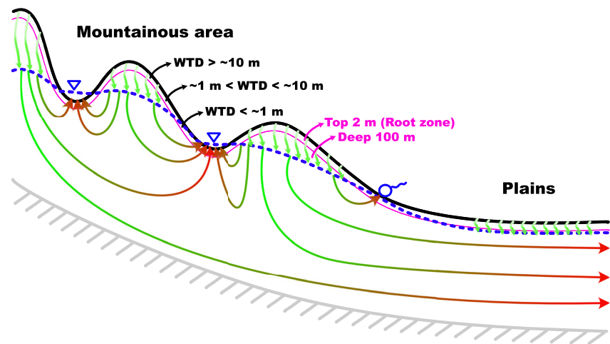
Figure 4. Conceptual diagram of topography-driven flow paths in the modeling domain based on the Tóthian concept. Mountainous areas and plains are dominated by rolling and flat topographies, respectively. The top 2 m represents the upper four layers of the model, that is, the root zone. The deeper 100 m is the bottom layer of the model. Three subregions in the mountainous areas differentiated by water table depth (WTD) are exemplified. These subregions represent the ridges with WTD larger than \sim 10 m, the hillslopes with WTD between \sim 1 m and \sim 10 m, and the valleys with WTD smaller than \sim 1 m.
