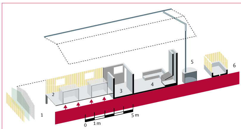
Figure 1: The prototype houses
