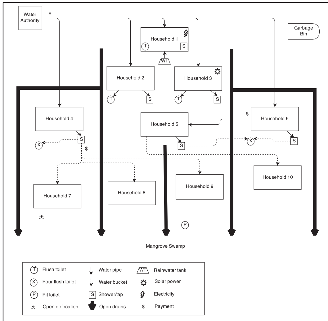
Fig. 2. Community water and sanitation systems map.
